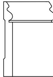
CT-240 5/8" x 5-1/4" CT-241 5/8" x 6-1/4" CT-242 5/8"x7-1/4"
