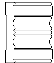
CT-137 7/8" X 5"
