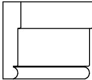
CT-155 3/4" X 3-1/4"
