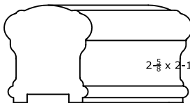
CT-6011 CT-6011-P(1/4" x 1-1/4") 2-5/8" x 2-15/16 (P- With Plow)
