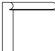
(Siding) CT-812C 5/8" X 7 1/4"
