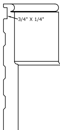
CT-831D 1" X 8-5/8"
