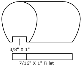
CT-6801 2 1/2" X 2 7/8"
