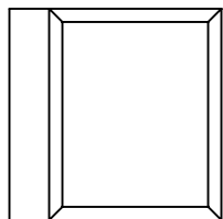
Plinth Block CT-882 1" Thick 3-1/4" to 4-1/2" Wide Specify Length
