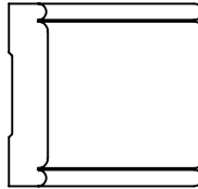
CT-640 3/4" X 3-1/2"
