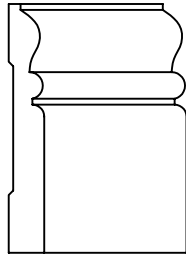
CT-202 11/16" X 3-1/2"
