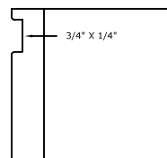
SQUARE STOCK WITH DADO
